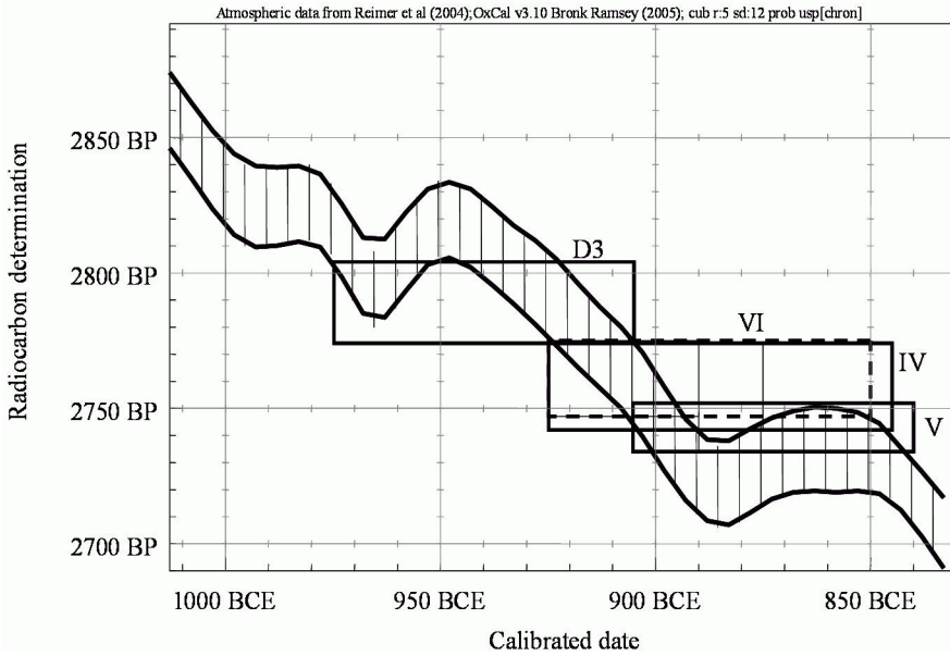
Figure 1 The full 1- \sigma range for Tel Rehov strata D-3 to IV (Table 2) superimposed on the IntCal04 calibration curve (Reimer et al. 2004).
